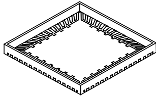
56L - 8X8mm PITCH 0.5mm
