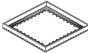
64L - 9X9mm PITCH 0.5mm
