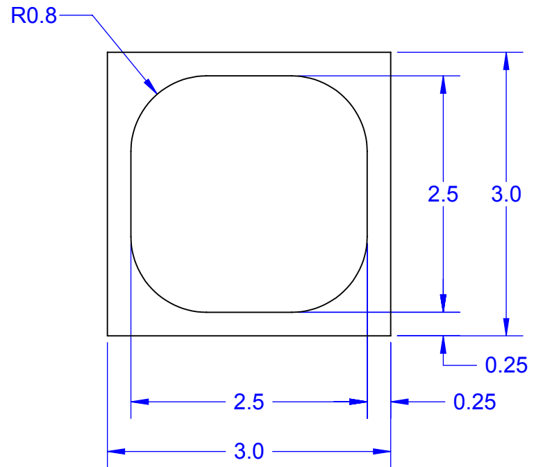
BOTTOM VIEW OPEN SIDE
