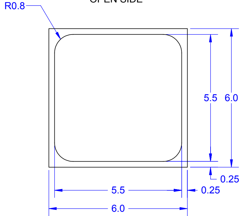
BOTTOM VIEW OPEN SIDE
