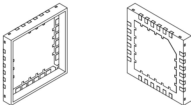
ISOMETRIC VIEW OF CAVITY SIDE
