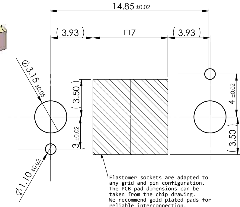
PCB LAYOUT
