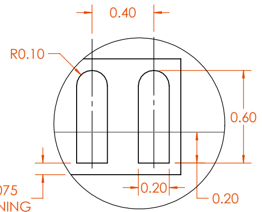
DETAIL A SCALE 40 : 1
